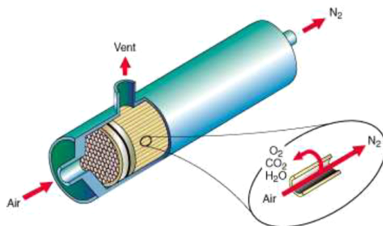
Figure 2 - Separating nitrogen through the membrane
