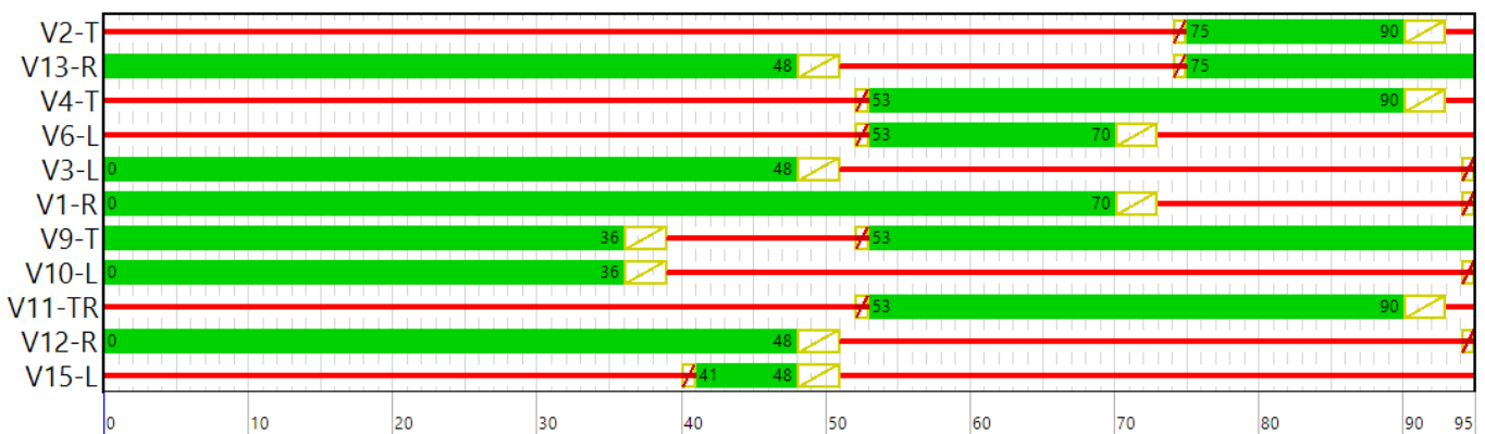
Figure 8 Revised signal control plan
