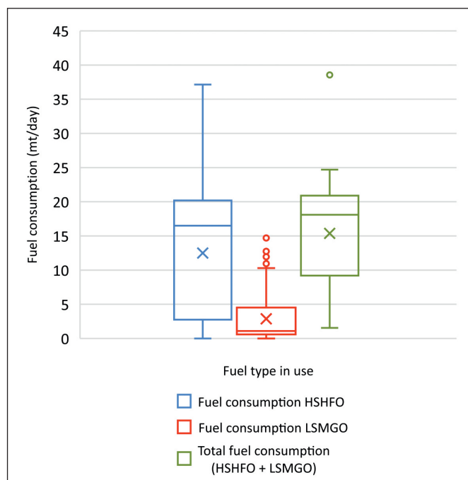
Figure 2 Box plot of averages, quartiles and max. daily fuel consumption over a complete period 02/2020 – 08/2020 – M/V Vessel
