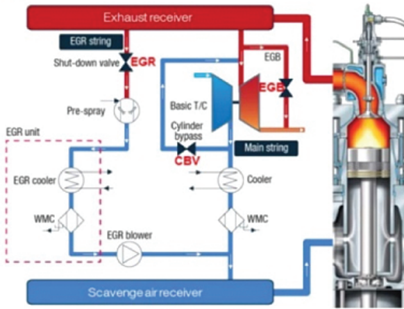
Fig. 8 Schematic diagrams of different variants of EGR systems: a) EGRBP, b) EGRTC [2]
