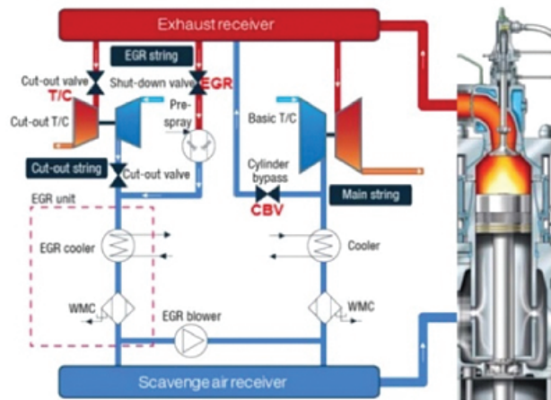
Fig. 8 Schematic diagrams of different variants of EGR systems: a) EGRBP, b) EGRTC [2]
