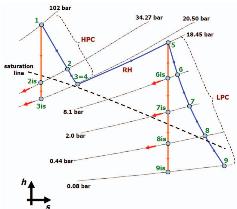
Fig. 2 Steam expansion processes (real - blue curves; ideal - orange lines) in h-s diagram for the analyzed steam turbine
