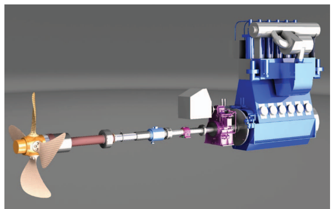
Figure 1 Typical Ship Propulsion System Elements Rendering
