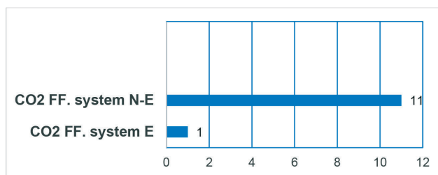
Figure 3 CO 2 firefighting system efficiency (N-E – Not Effective, E – Effective) as elaborated from the investigation reports.
