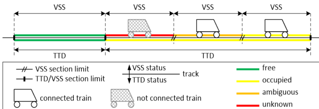
Figure 5. Marking of VSS subsection (Hybrid ERTMS/ETCS Level 3, Principles).
