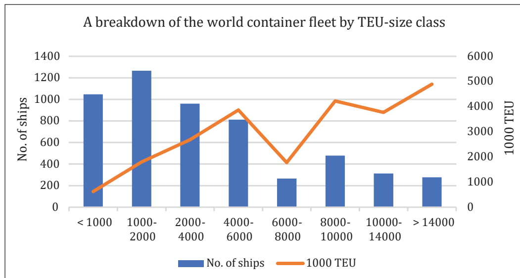
Figure 2 World fully-cellular container fleet by TEU-size class (situation on 01.01.2021, based on [30])
